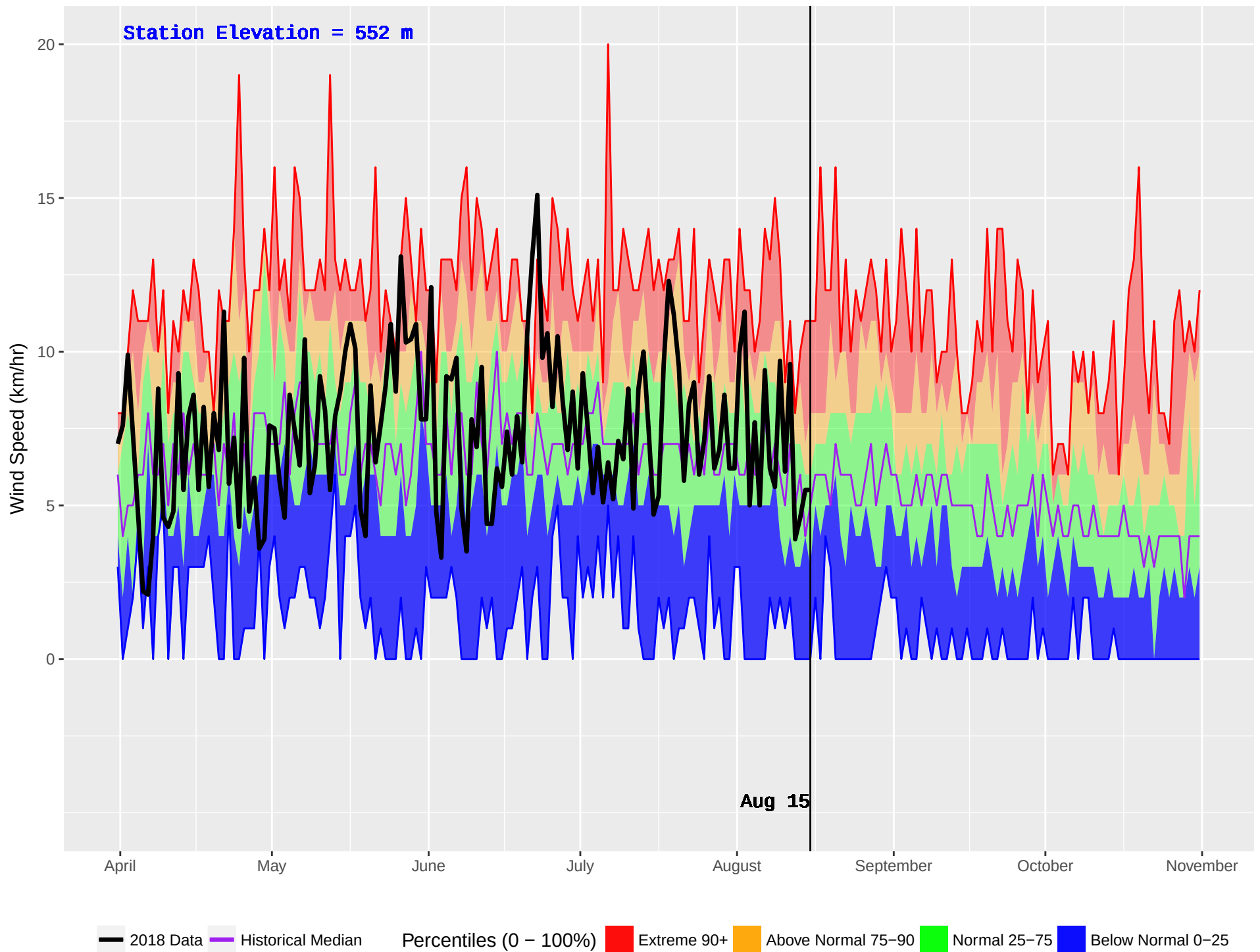
NAHATLATCH (316) : Historical (2001–2016) and Current (2018) Daily Wind Speed
