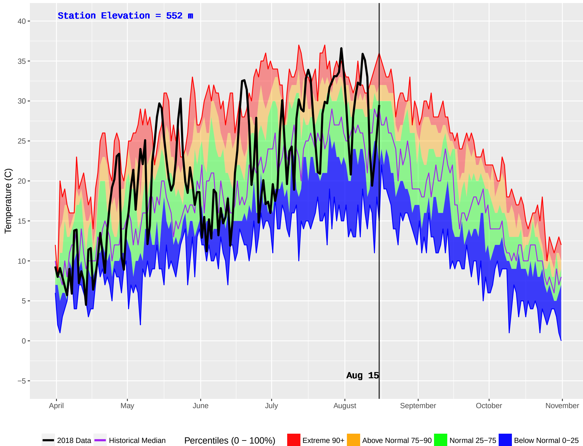
NAHATLATCH (316) : Historical (2001–2016) and Current (2018) Daily Temperature
