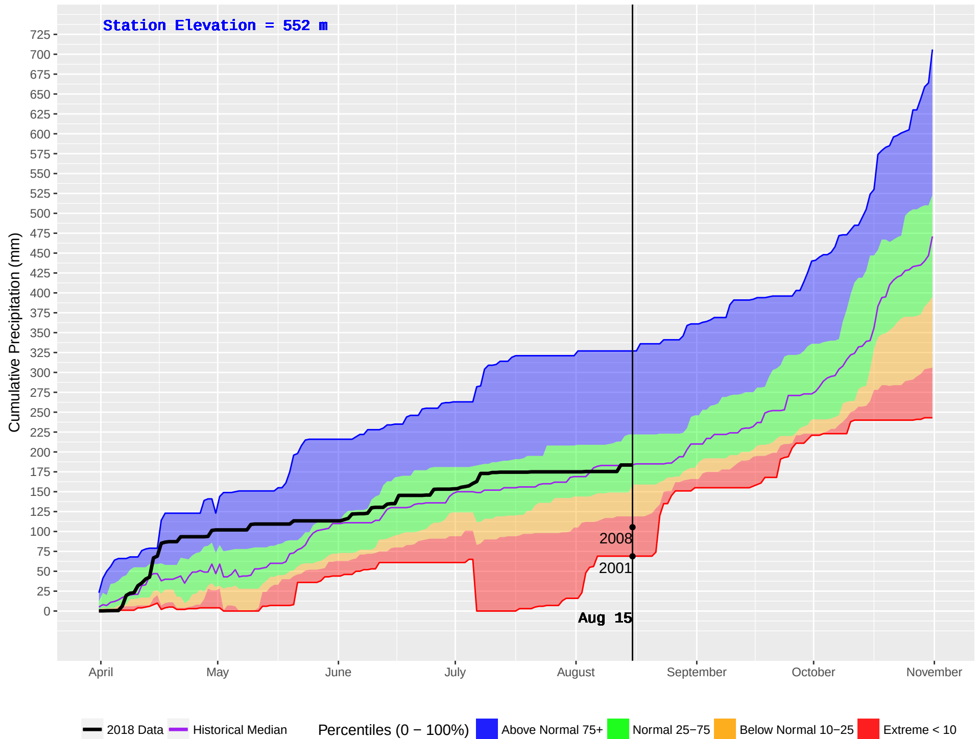
NAHATLATCH (316) : Historical (2001–2016) and Current (2018) Daily Cumulative Precipitation
