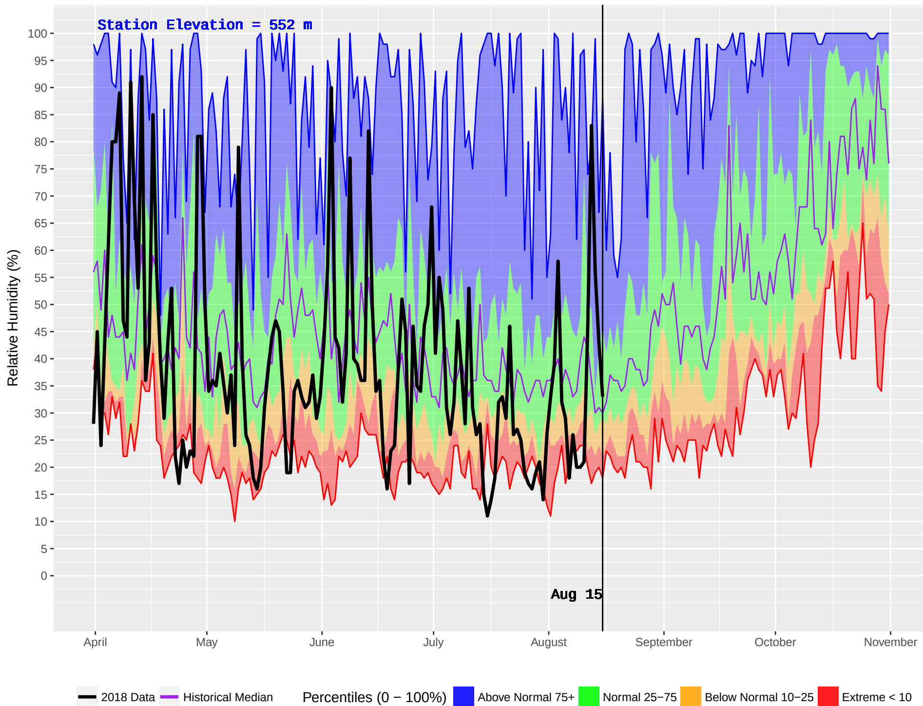
NAHATLATCH (316) : Historical (2001–2016) and Current (2018) Daily Relative Humidity
