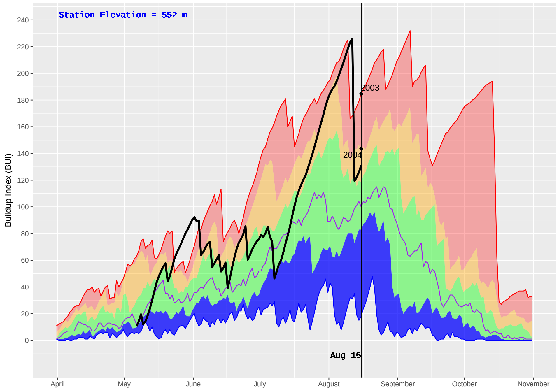
NAHATLATCH (316) : Historical (2001–2016) and Current (2018) Daily Buildup Index (BUI)
