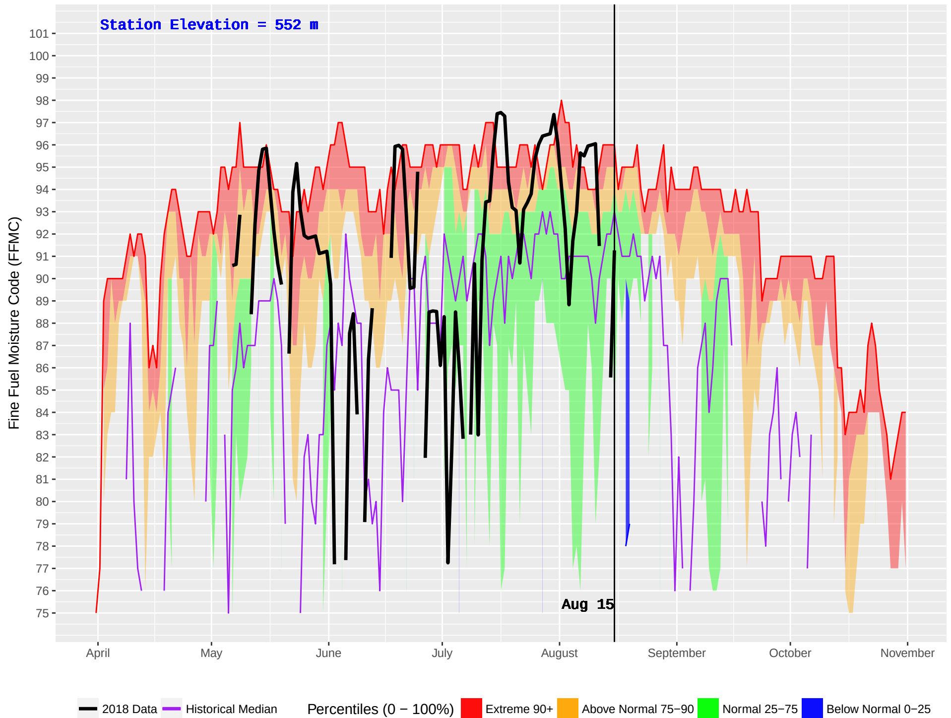
NAHATLATCH (316) : Historical (2001–2016) and Current (2018) Daily Fine Fuel Moisture Code (FFMC)
