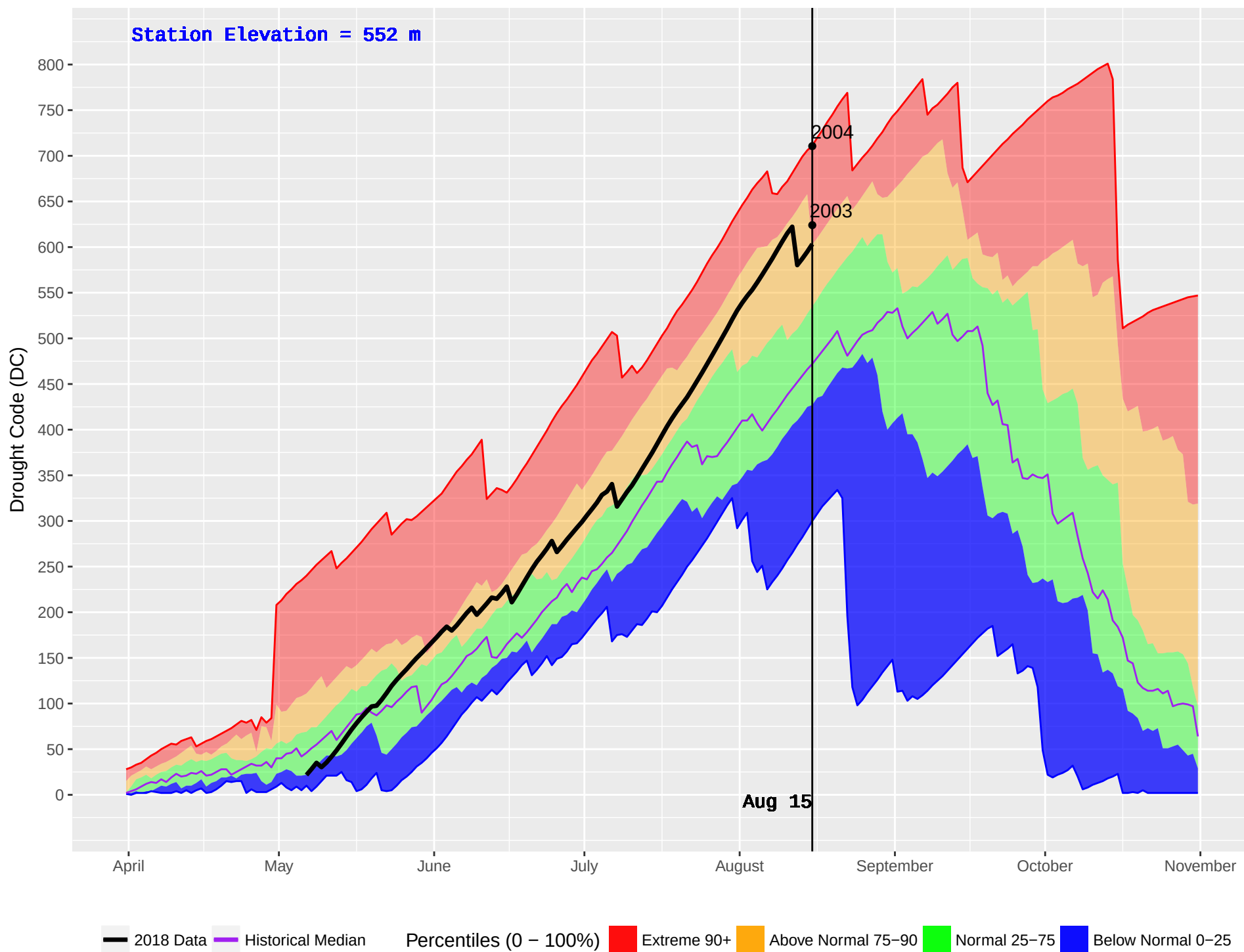
NAHATLATCH (316) : Historical (2001–2016) and Current (2018) Daily Drought Code (DC)
