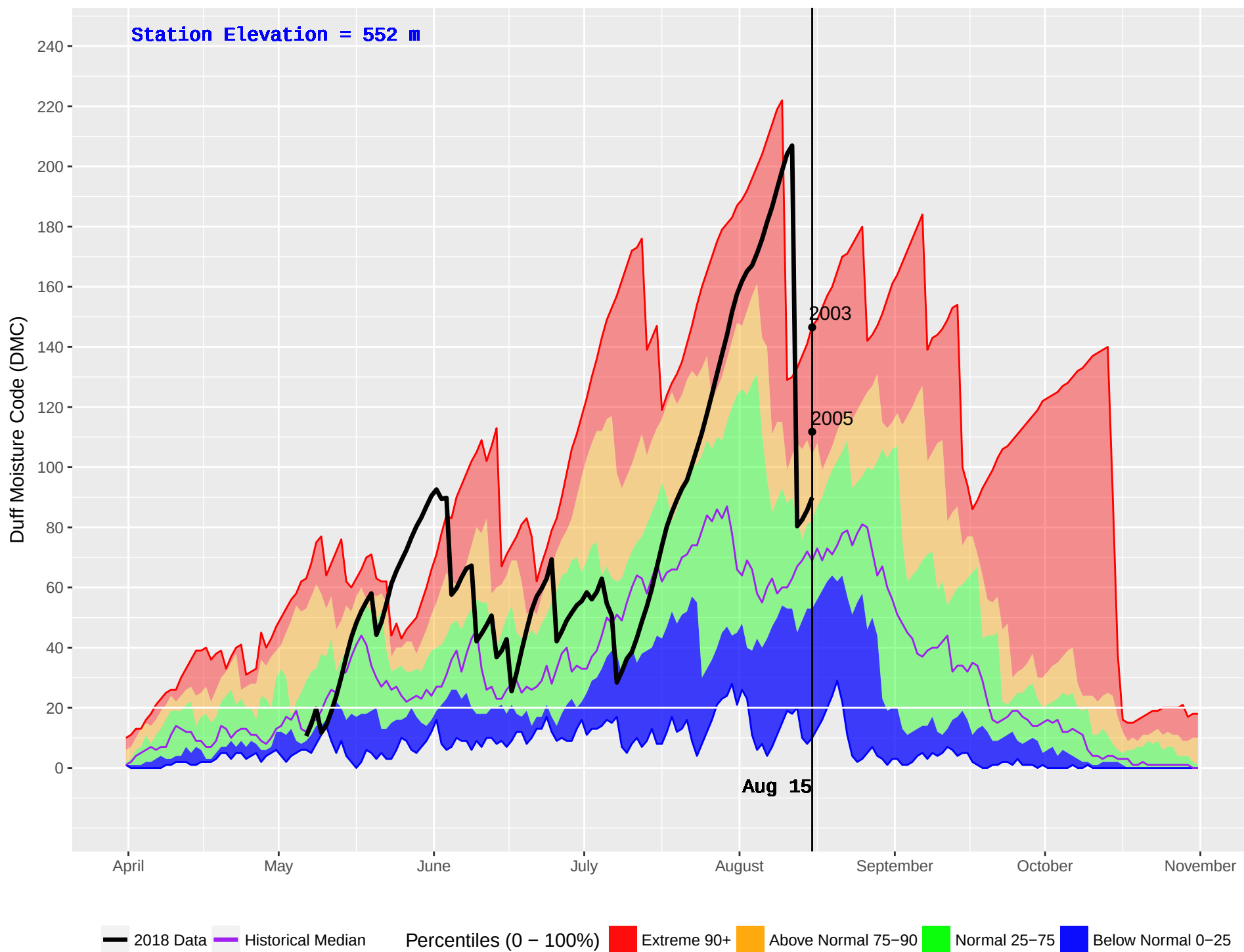
NAHATLATCH (316) : Historical (2001–2016) and Current (2018) Daily Duff Moisture Code (DMC)
