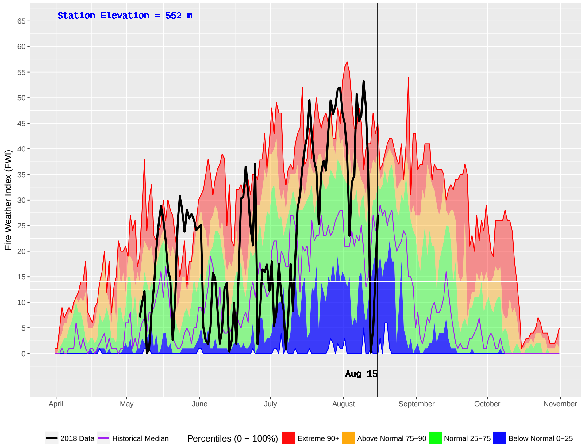
NAHATLATCH (316) : Historical (2001–2016) and Current (2018) Daily Fire Weather Index (FWI)
