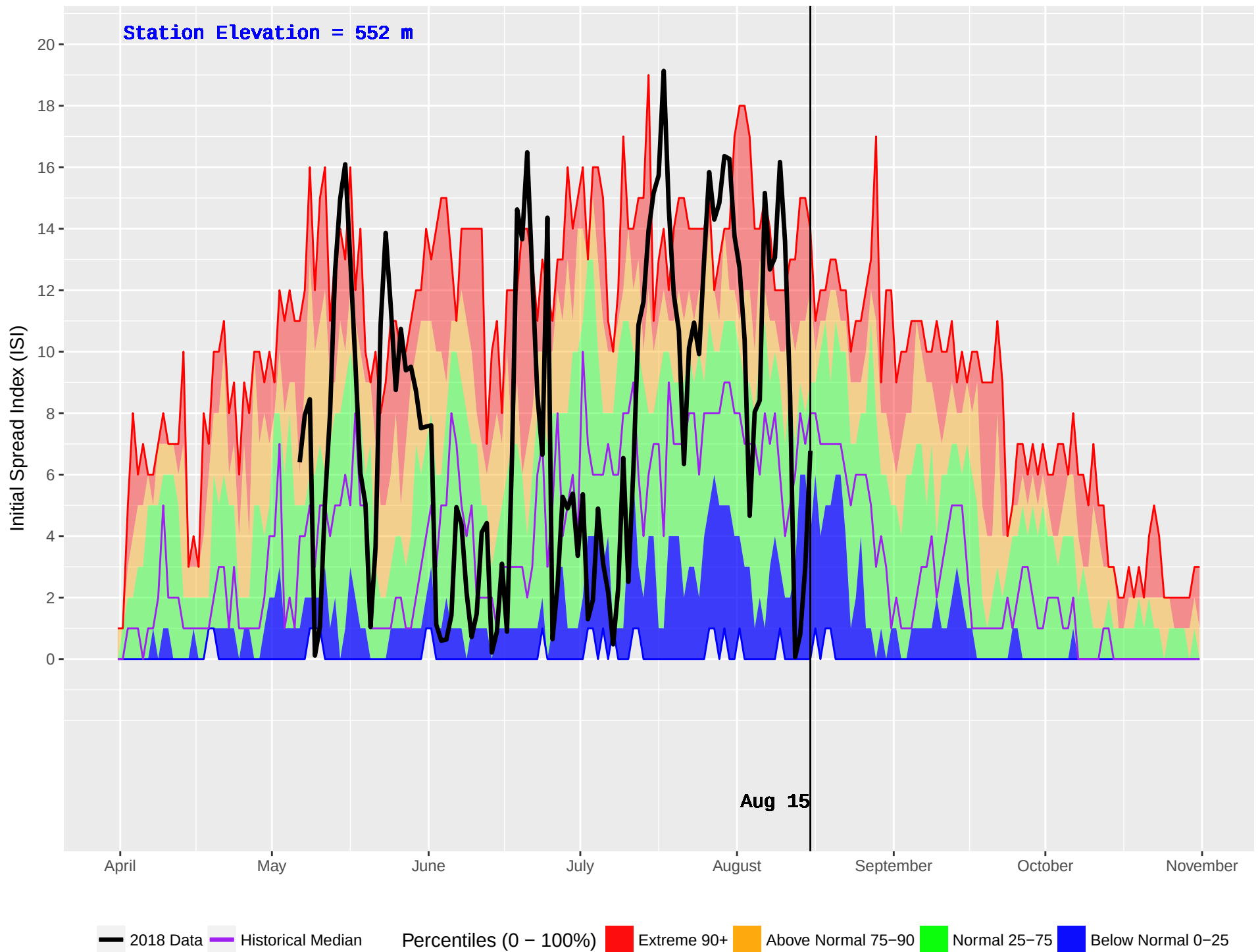
NAHATLATCH (316) : Historical (2001–2016) and Current (2018) Daily Initial Spread Index (ISI)
